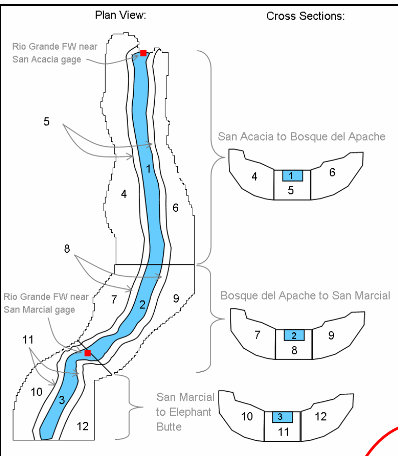
Socorro GW Basin (based on Shafike 2005 model)
