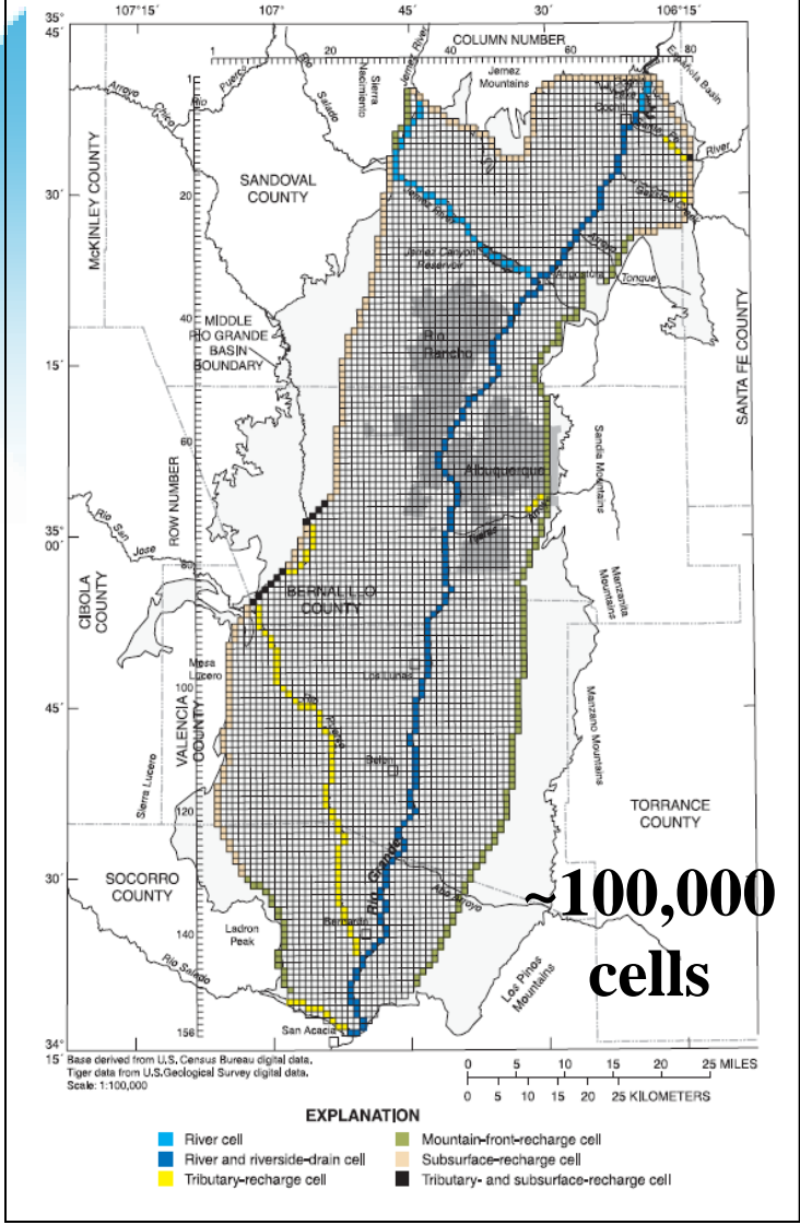
McAda and Barroll 2002, Figure 7. Albuquerque Basin MODFLOW model extnt.
