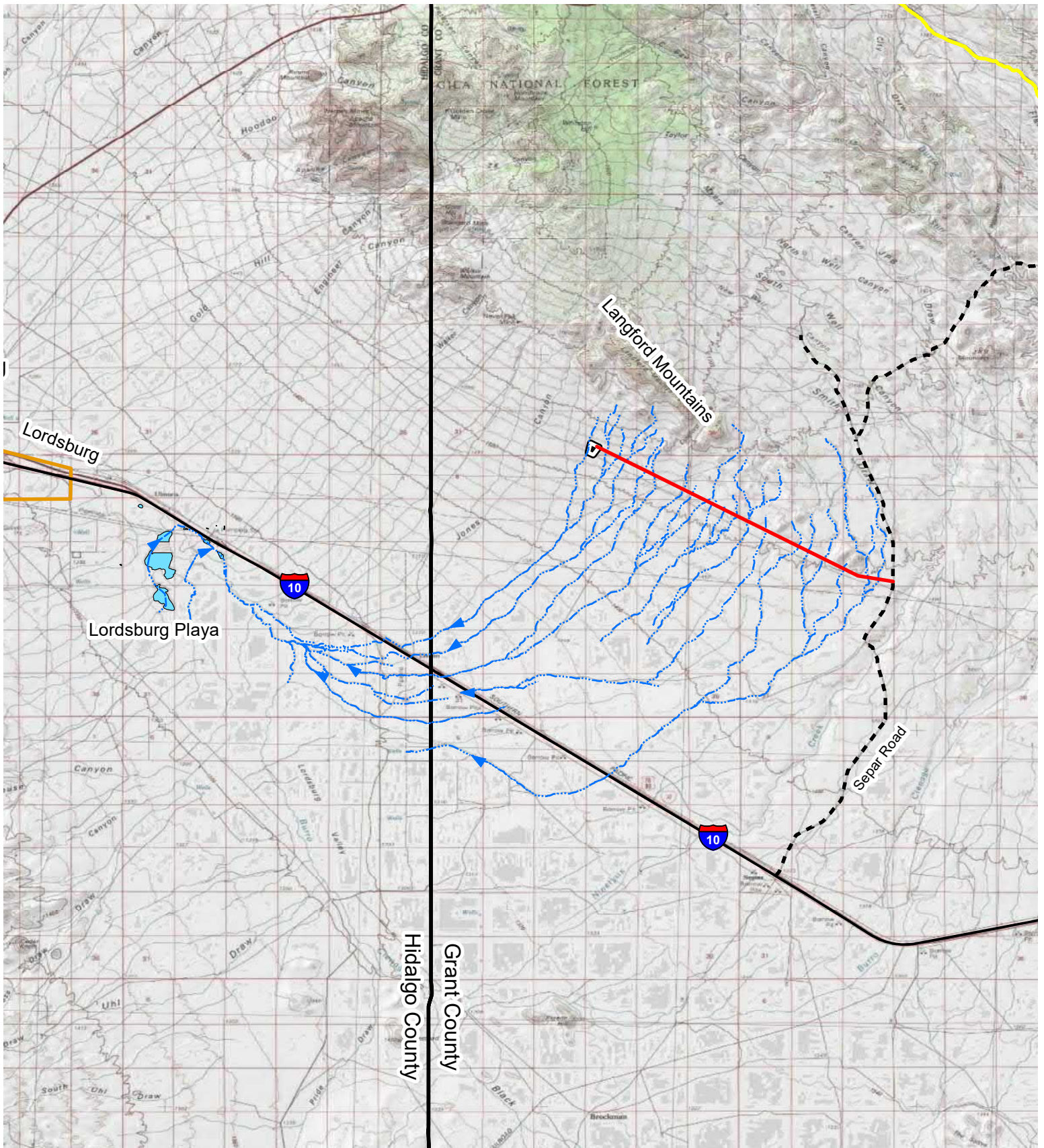
Figure 2: Drainage Characteristics
